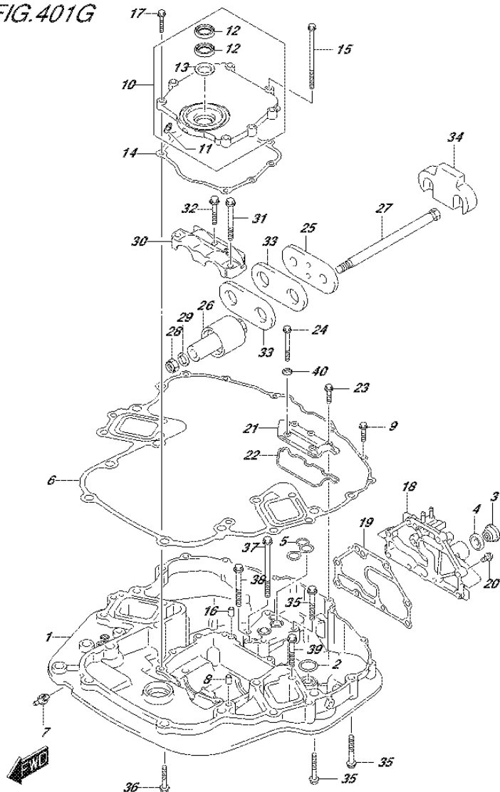
FIG.401G (3-D-13) ENGINE HOLDER (DF225Z E01)
