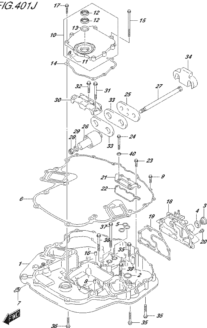
FIG.401J (3-E-3) ENGINE HOLDER (DF250T E01)
