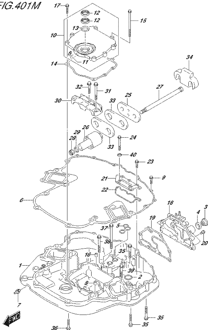
FIG.401M (3-E-9) ENGINE HOLDER (DF250Z E40)
