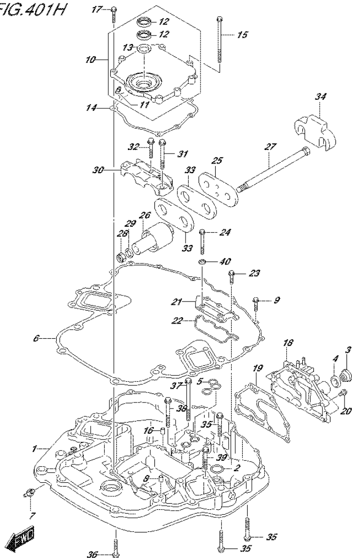
FIG.401H (3-D-15) ENGINE HOLDER (DF225Z E40)
