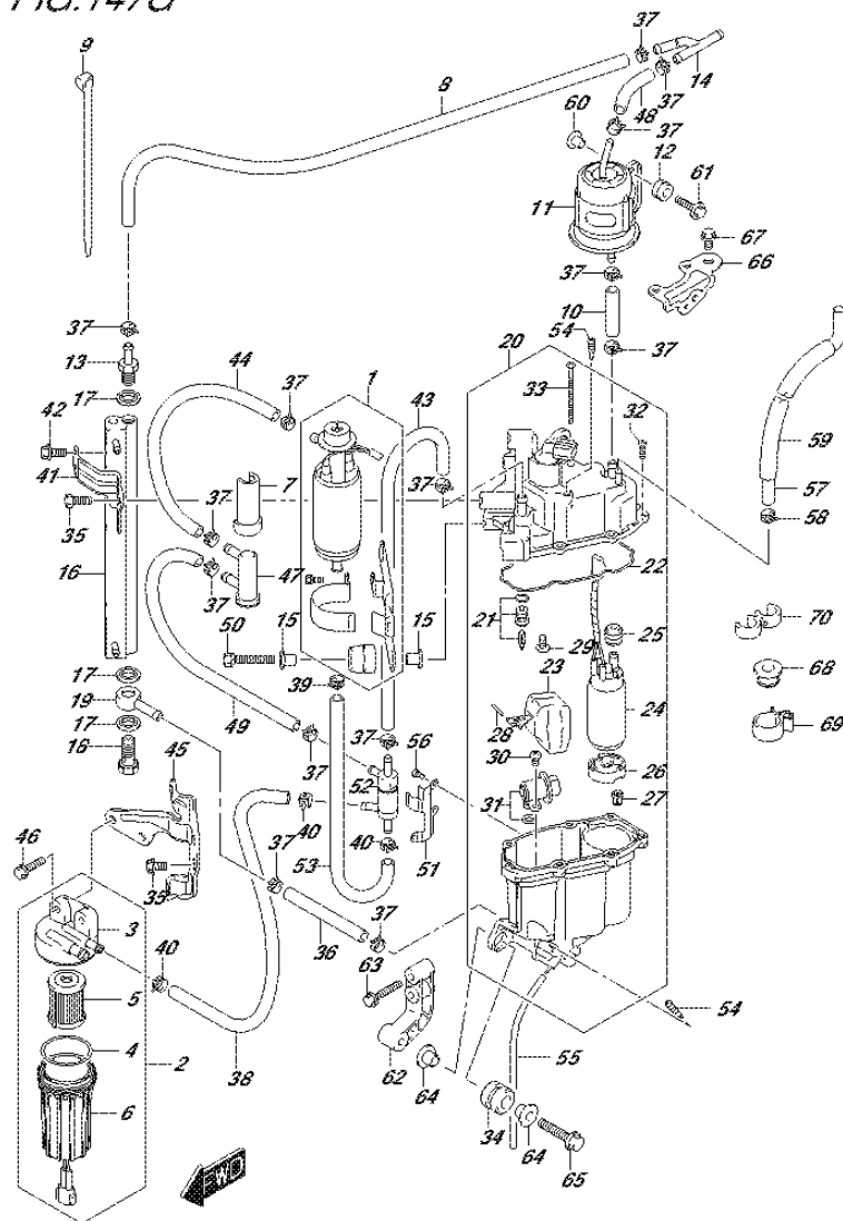
DF225Z_E01_017_147G FUEL PUMP/FUEL VAPOR SEPARATOR
