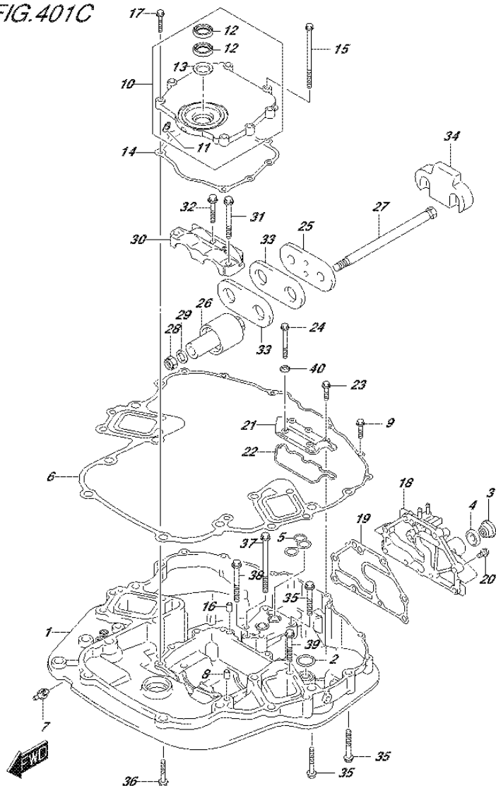
FIG.401C (3-D-5) ENGINE HOLDER (DF200Z E01)
