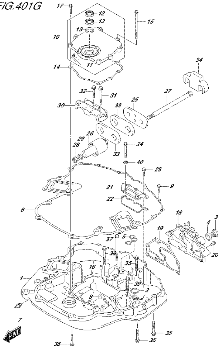
FIG.401G (3-D-12) ENGINE HOLDER (DF225Z E01)
