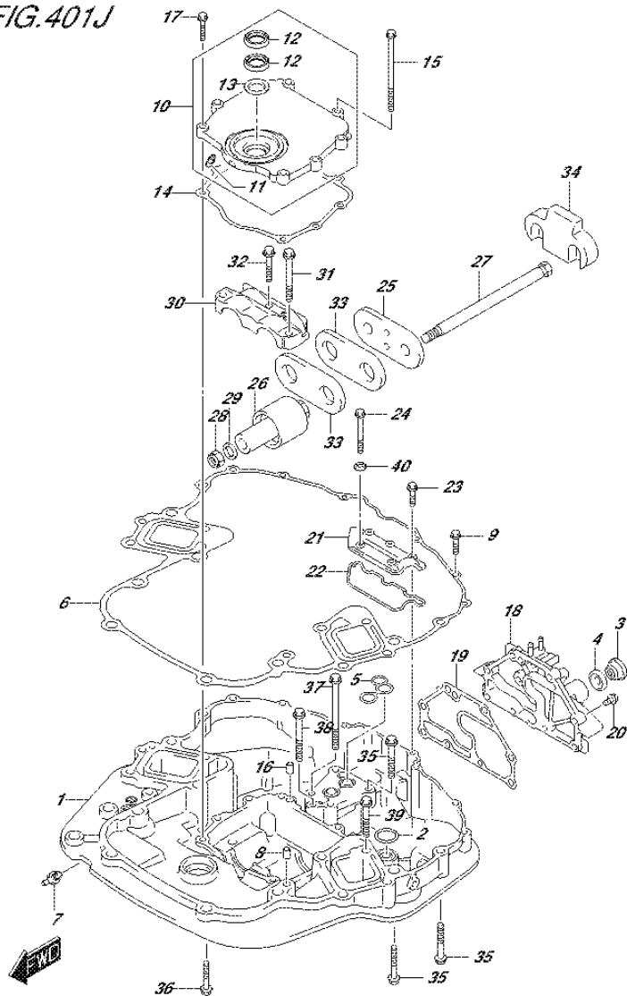
FIG.401J (3-E-2) ENGINE HOLDER (DF250T E01)
