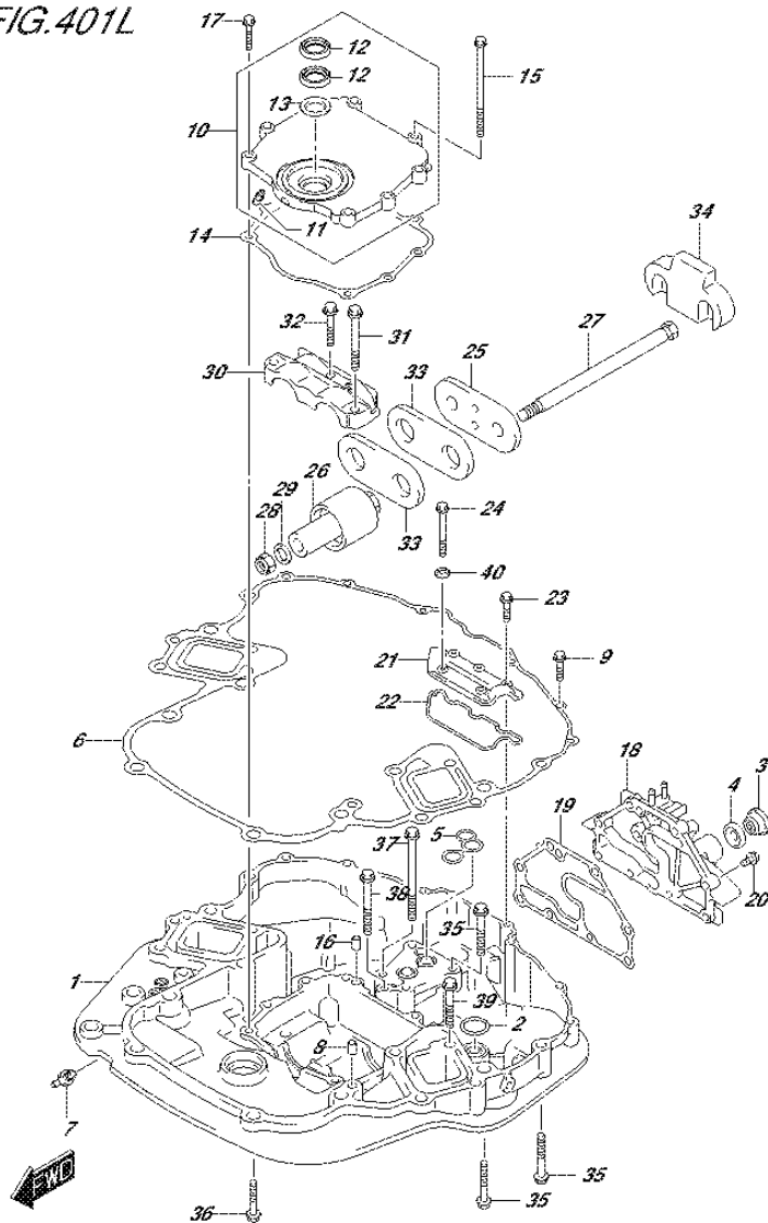
FIG.401L (3-E-6) ENGINE HOLDER (DF250Z E01)
