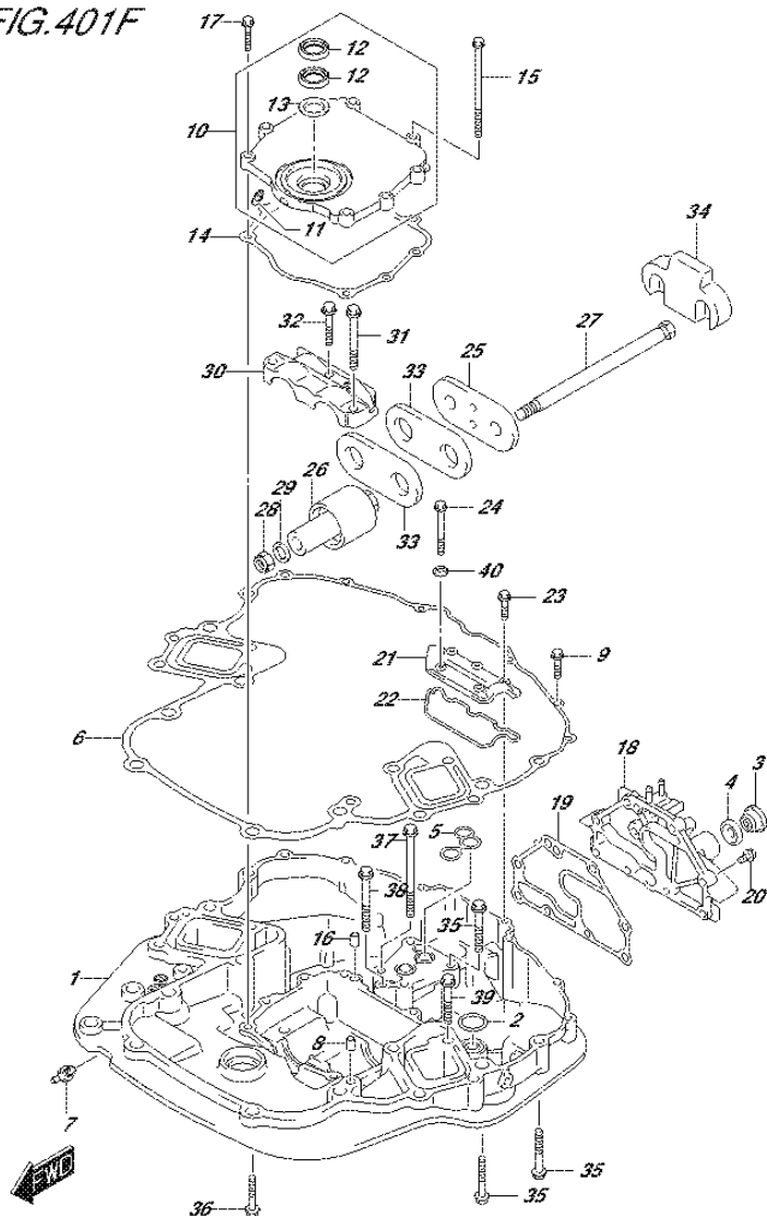
FIG.401F (3-D-11) ENGINE HOLDER (DF225T E40)
