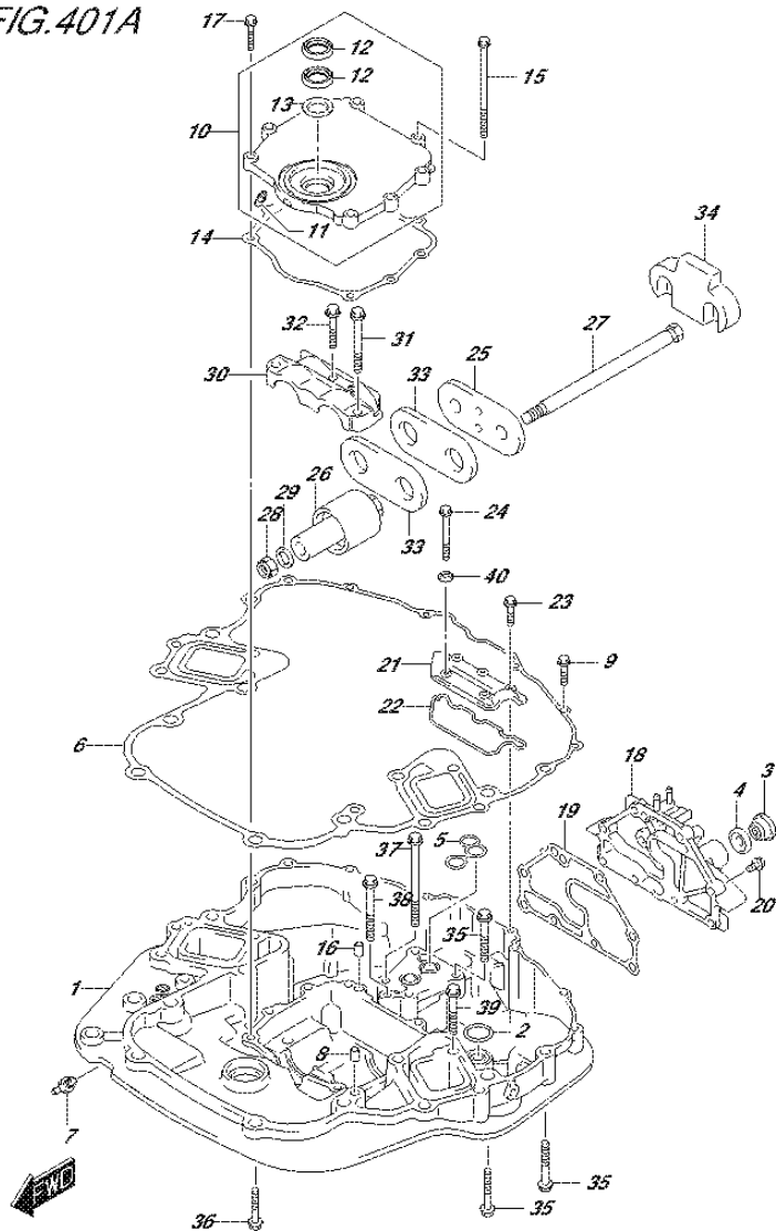
FIG.401A (3-C-15) ENGINE HOLDER (DF200T E01)
