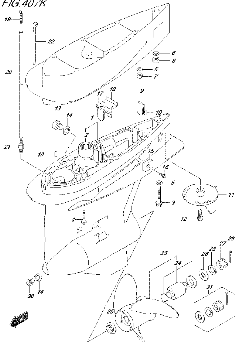
DF250_E01_017_407K GEAR CASE
