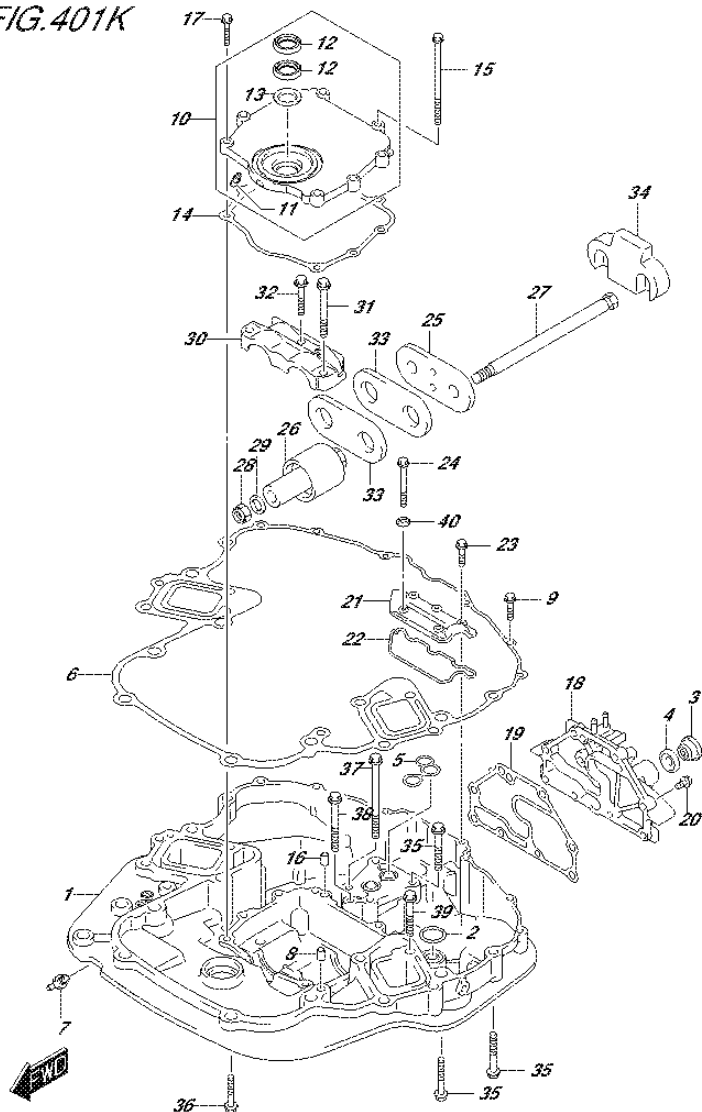
FIG.401K (3-E-5) ENGINE HOLDER (DF250T E40)
