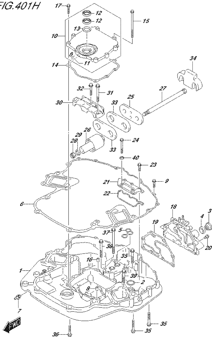
FIG.401H (3-D-14) ENGINE HOLDER (DF225Z E40)
