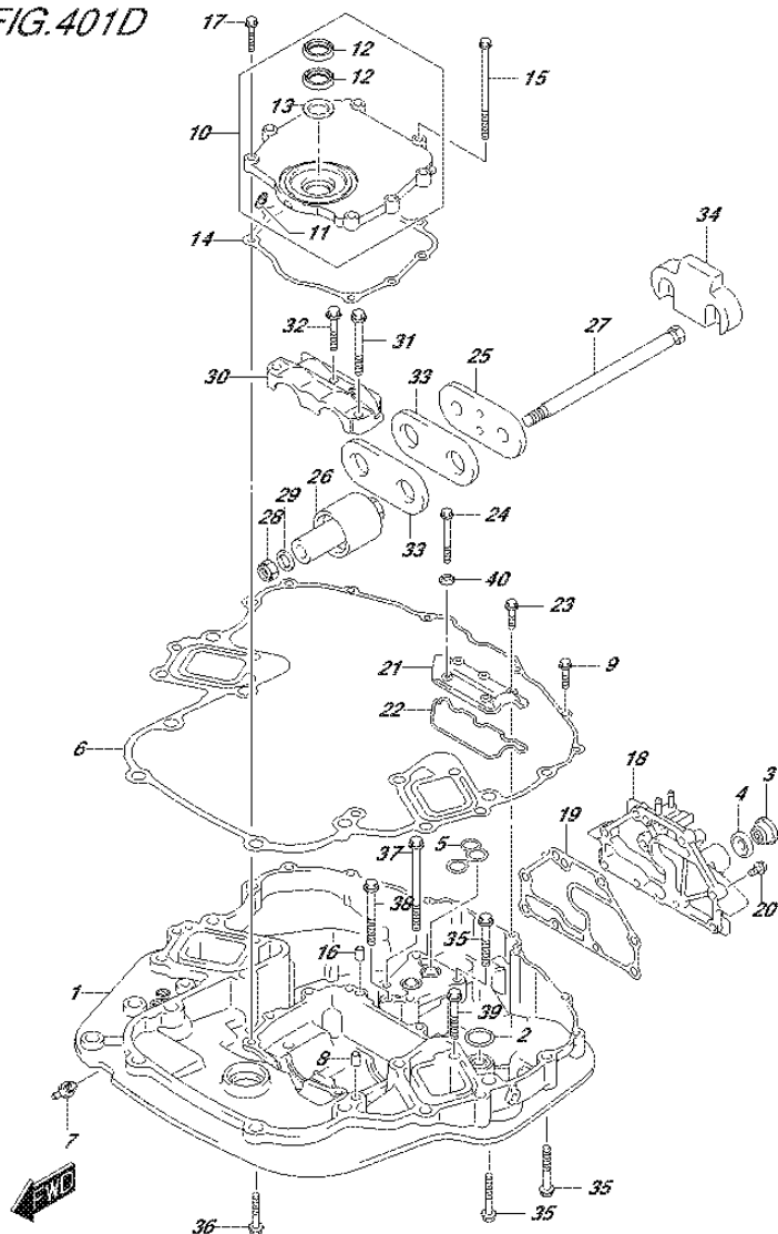
FIG.401D (3-D-6) ENGINE HOLDER (DF200Z E40)
