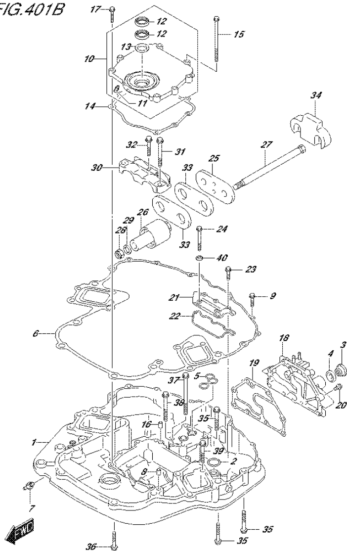
FIG.401B (3-D-3) ENGINE HOLDER (DF200T E40)
