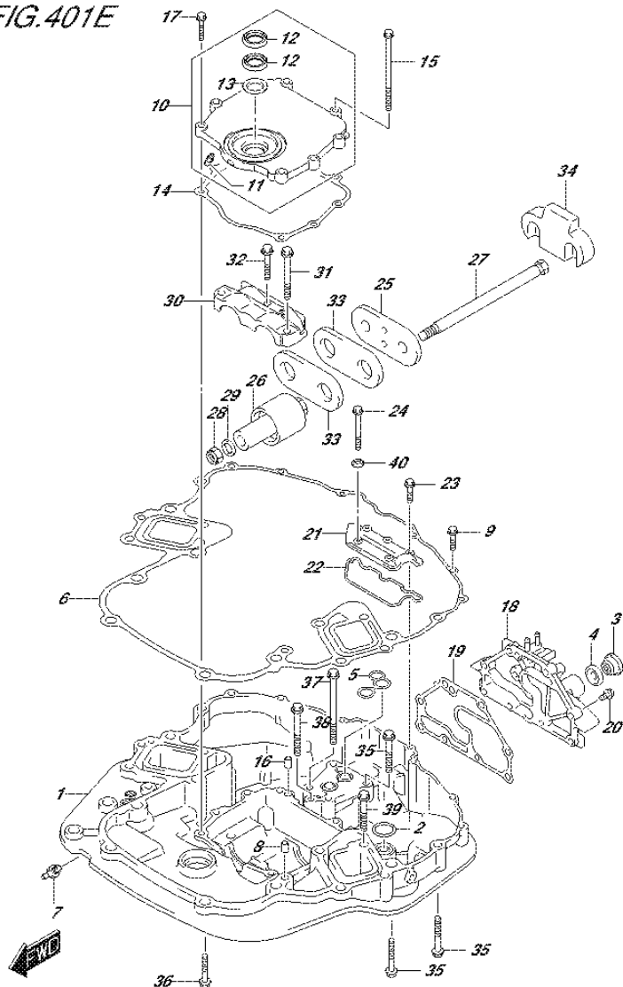
FIG.401E (3-D-9) ENGINE HOLDER (DF225T E01)
