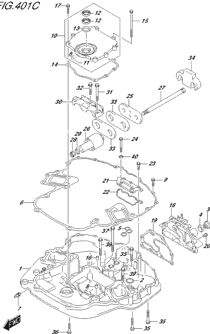
FIG.401C (3-D-4) ENGINE HOLDER (DF200Z E01)
